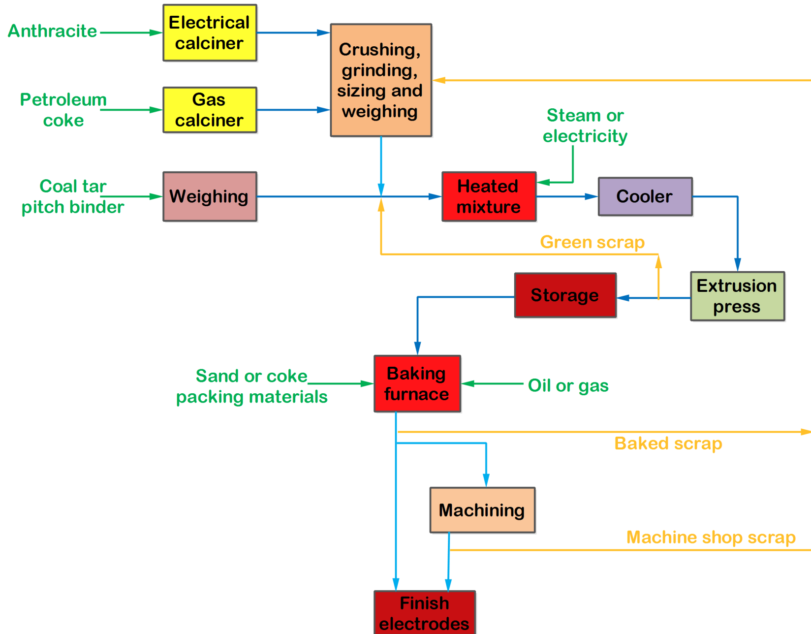
Figure: Manufacture of Carbon electrode from petroleum coke and anthracite
